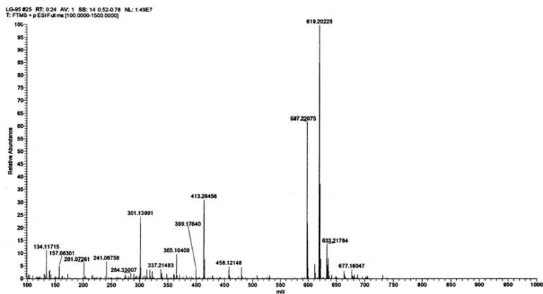
2-rasm. Namunaga Na + ion qo'shib olingan mass-spektr
