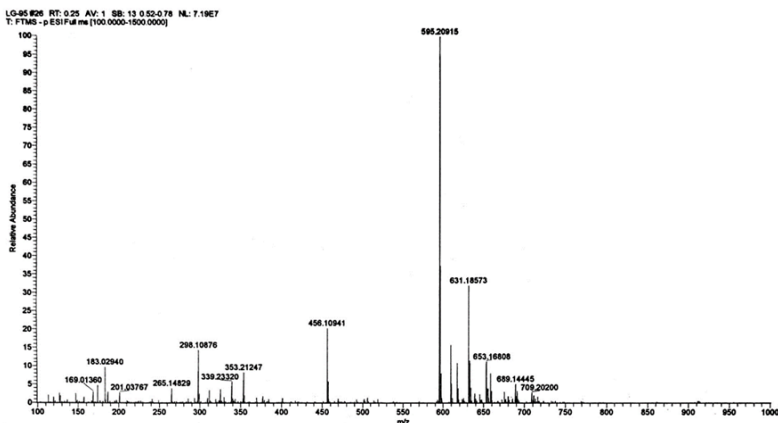
1-rasm. Elektrosprey usuli bilan ionlashtirib olingan namunaning fur'e-almashtirish FTMS usuli bilan o'lchangan mass-spektri
